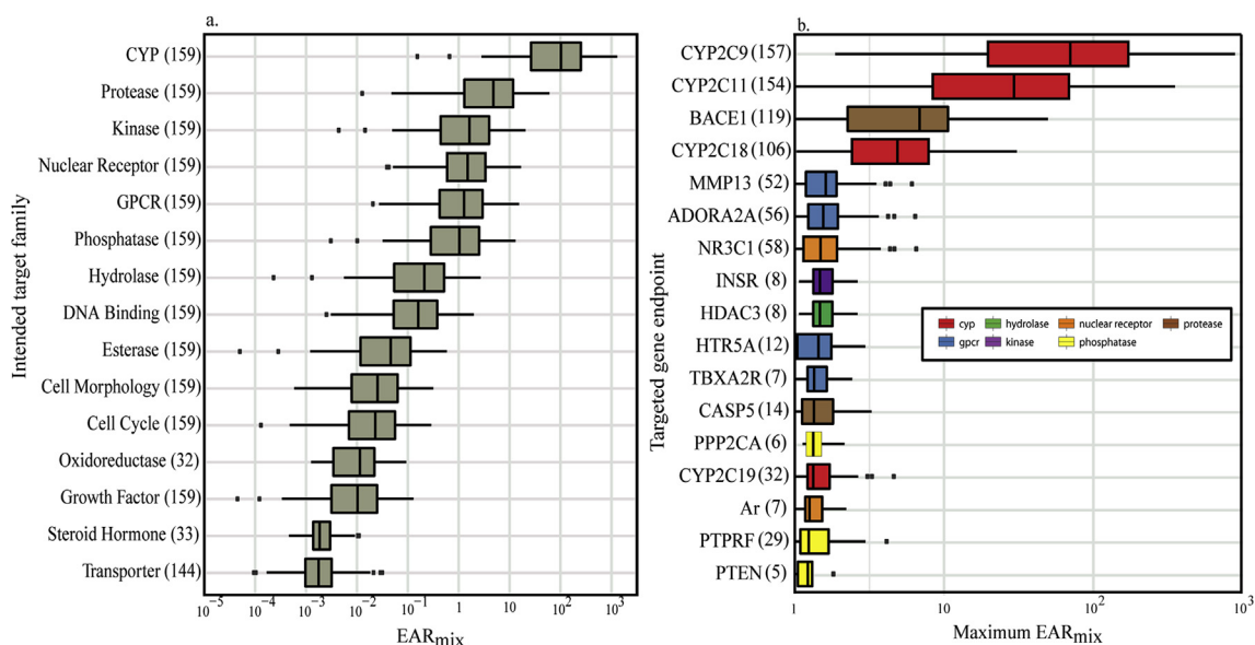
Fig. 3. Summaries of mixture exposure–activity ratios ( EAR_{mix} ) for organic contaminants detected in eaglet plasma collected from six study areas in the upper Midwestern United States, 2006–2015. Mixture EAR was calculated by summing the calculated EAR for every chemical identified as potentially affecting specific (a) intended target families and (b) targeted gene endpoints. For brevity, Fig. 3b only shows identified gene targets with an associated EAR_{mix} \geq 1 and sample size \geq 5 . Numbers in parentheses after target family or endpoint name represent the number of sites (eagle nests) affected. Boxplot whiskers extend to the smaller of the maximum value and 1.5 times the interquartile range, and the larger of the minimum value and 1.5 times the interquartile range. Individual points represent values beyond the ends of the whiskers.
