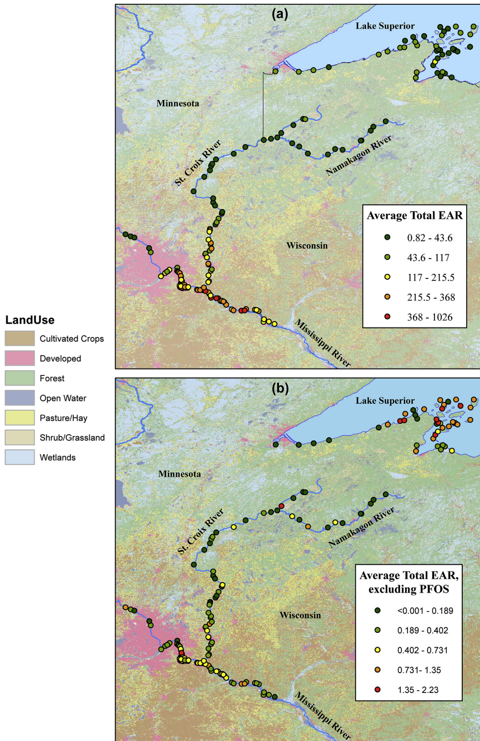
Fig. 4. Average total exposure—activity ratios (EAR) (a) including PFOS, and (b) excluding PFOS in bald eagle plasma samples collected from six study areas in the upper Midwestern United States, 2006–2015. Total EAR values represent all chemicals detected within a sample for which activity concentrations exist.
