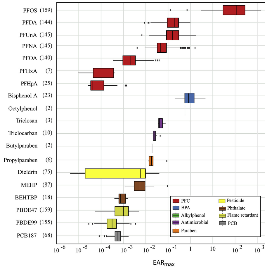
Fig. 2. Chemical summaries of maximum exposure–activity ratios ( EAR_{max} ) for organic contaminants detected in eaglet plasma collected from six study areas in the upper Midwestern United States, 2006–2015. Values represent the maximum of the sum of EAR for all organic contaminant–endpoint matches for a given chemical within a sample. Numbers in parentheses after chemical name represent the number of sites (eagle nests) at which the chemical was detected. Boxplot whiskers extend to the smaller of the maximum value and 1.5 times the interquartile range, and the larger of the minimum value and 1.5 times the interquartile range. Individual points represent values beyond the ends of the whiskers. PFC, perfluorinated chemical; BPA, bisphenol A; PCB, polychlorinated biphenyl.
