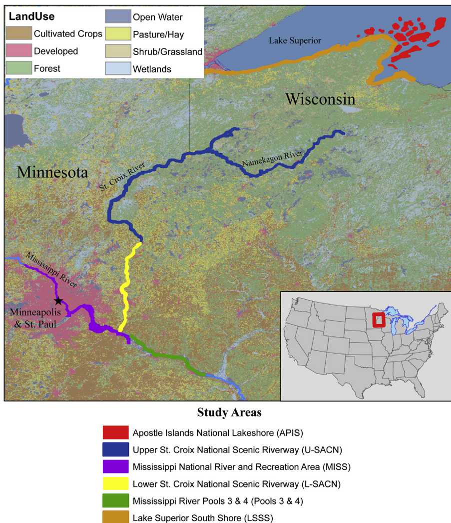
Fig. 1. Study areas where bald eaglet plasma was collected during 2006–2015.
